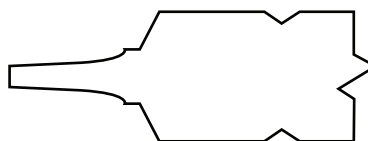
HIP/TRUE V-GROOVE PANEL 1 1/8", 1 3/8"
