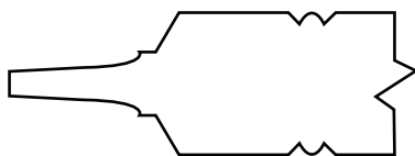
BEADED RAISED PANEL 1 1/8", 1 3/8"
